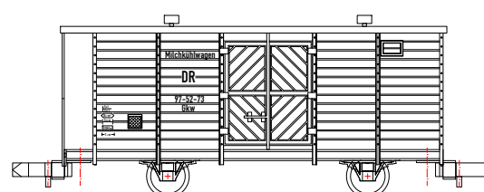
Gkw 97-52-73 "Milchkühlwagen" (ex. Pollo) Gww 97-51-87 "Milchkühlwagen"
