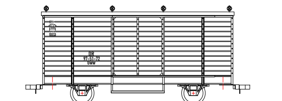
Gww 97-51-72 (ex. Pollo) Gww 97-51-57
